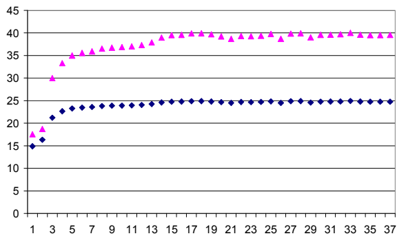
Figure 3: Fastest Vehicle Speed (◆, [ \text{m/s} ], y-axis) and Resulting Longest Braking Distance (▲, [m], y-axis) for a Complete Stop of the Vehicle Found in each Generation (x-axis) of the Evolutionary Testing
