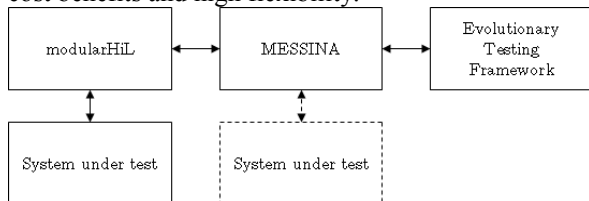
Figure 1: Components of the Test Automation Framework for Search-Based Testing (for testing in a MiL/SiL scenario no hardware-in-the-loop test system is needed, tests are directly executed by MESSINA)
