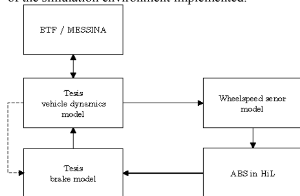
Figure 2: For testing the ABS system complex environment simulations are needed to simulate the wheelspeed sensor inputs for the ABS, the behaviour of the brakes and the vehicle dynamics
